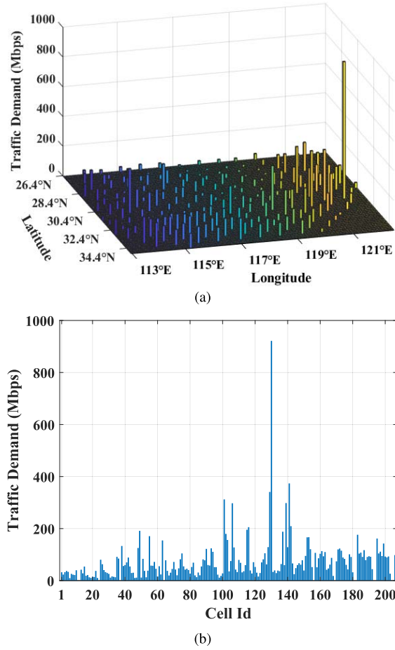
Fig. 8. Illustration of the traffic of each cell.
