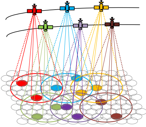
Fig. 1. Forward link of the multi-beam NGSO satellite communication system.
