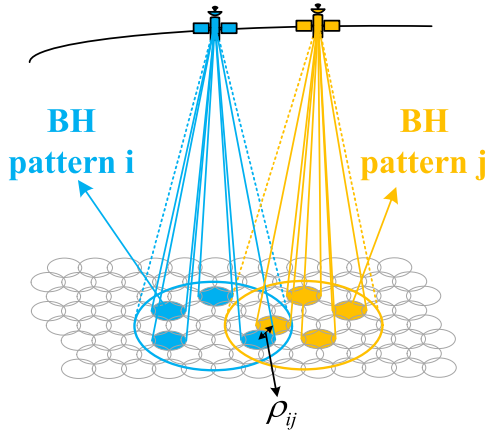
Fig. 6. Illustration of the spatial isolation between two beam hopping patterns.
