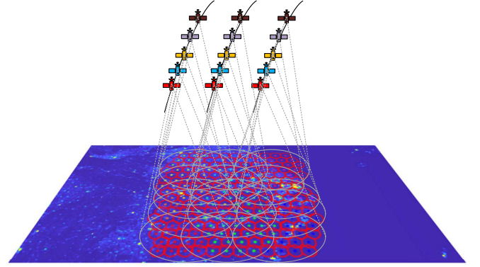
Fig. 7. Illustration of the coverage for 15 NGSO satellites.
