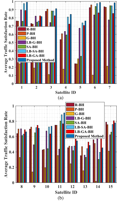
Fig. 10. Average traffic satisfaction rate of 15 satellites among different beam hopping algorithms.
