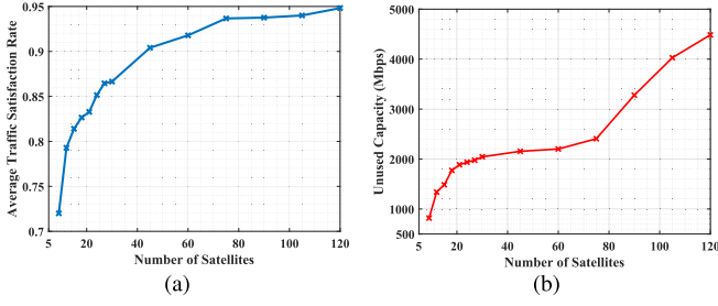
Fig. 12. Performance of the proposed algorithm for different number of satellites in terms of (a) average traffic satisfaction rate and (b) unused capacity.
