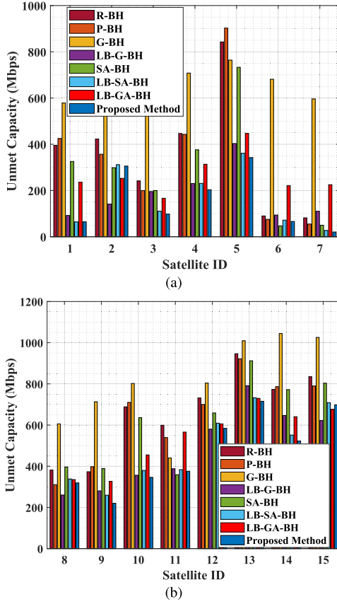
Fig. 11. Unmet capacity of 15 satellites among different beam hopping algorithms.
